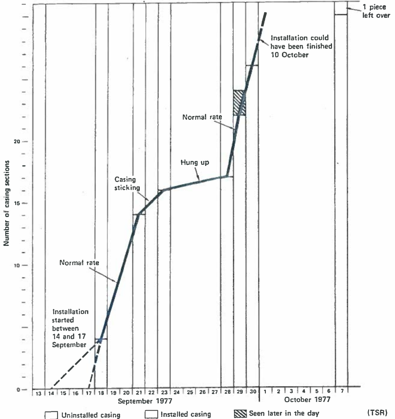
Figure 9. History of drill site casing installation.
